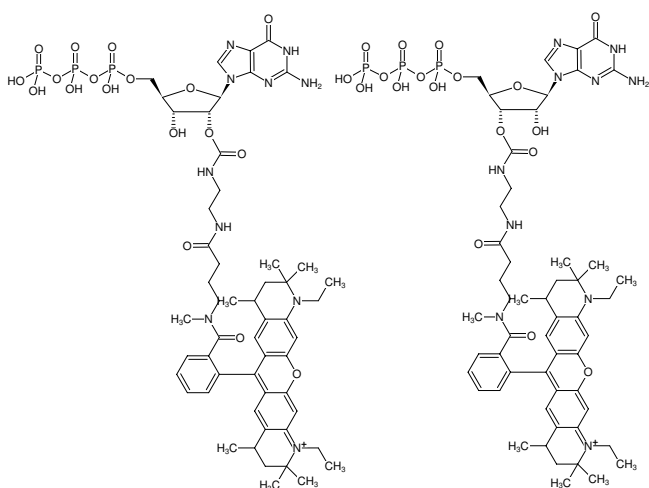
Structural formula of EDA-GTP-ATTO-Rho12
