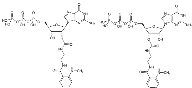
Structural formula of EDA-GTP-MANT
