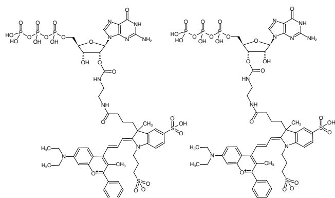
Structural formula of EDA-GTP-DYQ-661
