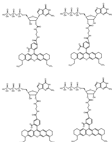
Structural formula of EDA-GTP-ATTO-565
