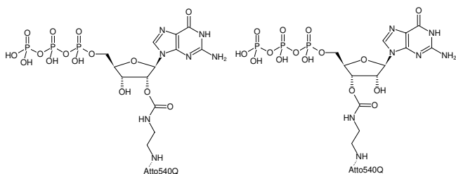
Structural formula of EDA-GTP-ATTO-540Q
