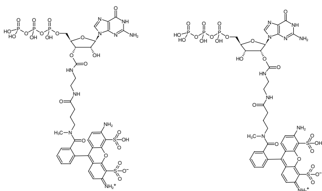
Structural formula of EDA-GTP-ATTO-488
