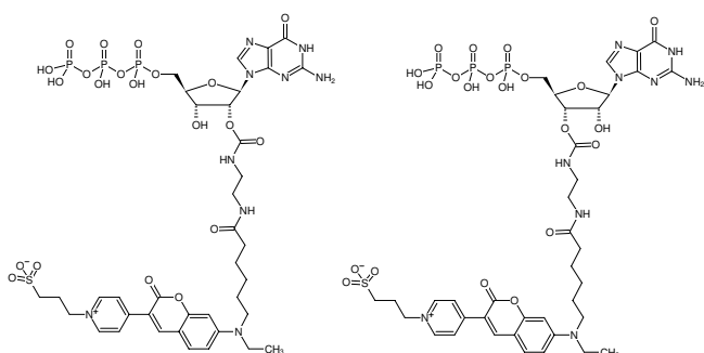
Structural formula of EDA-GTP-DY-485XL
