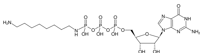
Structural formula of \gamma -[(8-Aminoethyl)-imido]-GTP
