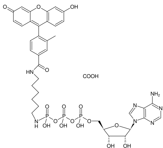
Structural formula of \gamma -[(6-Aminohexyl)-imido]-ATP-5-FAM
