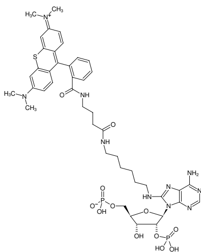
Structural formula of 8-(6-Aminoethyl)-amino-adenosine-2',5'-bisphosphate-ATTO-Thio12
