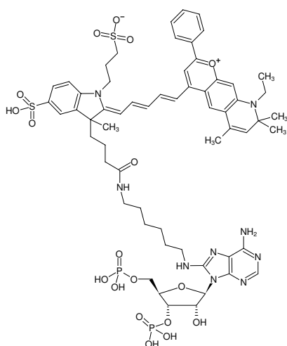
Structural formula of 8-(6-Aminoethyl)-amino-adenosine-3',5'-bisphosphate-DY-776
