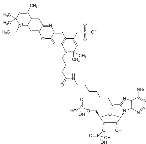
Structural formula of 8-(6-Aminoethyl)-amino-adenosine-3',5'-bisphosphate-ATTO-700
