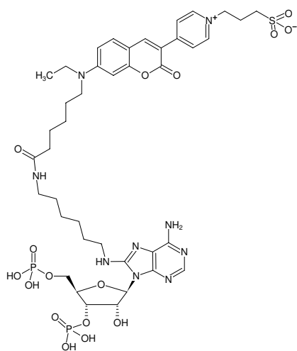
Structural formula of 8-(6-Aminoethyl)-amino-adenosine-3',5'-bisphosphate-DY-485XL
