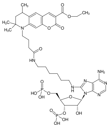
Structural formula of 8-(6-Aminoethyl)-amino-adenosine-3',5'-bisphosphate-ATTO-425
