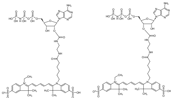
Structural formula of EDA-AppNHp (EDA-AMPPNP)-Cy5
