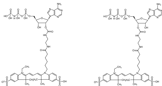
Structural formula of EDA-AppNHp (EDA-AMPPNP)-Cy3
