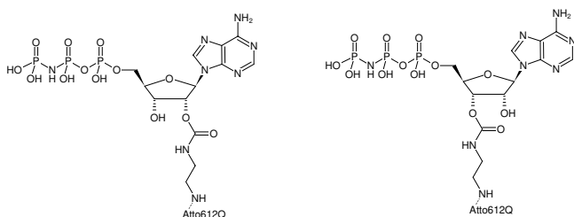
Structural formula of EDA-AppNHp (EDA-AMPPNP)-ATTO-612Q
