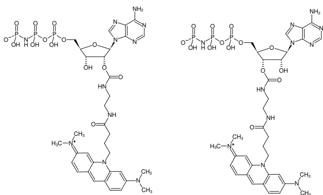
Structural formula of EDA-AppNHp (EDA-AMPPNP)-ATTO-495
