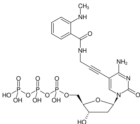
Structural formula of 5-Propargylamino-dCTP-MANT
