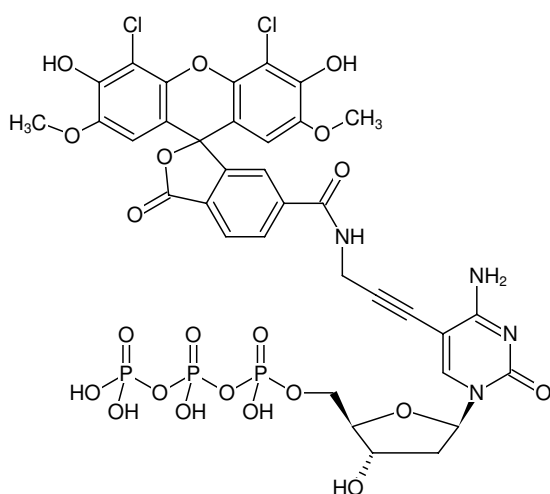
Structural formula of 5-Propargylamino-dCTP-6-JOE
