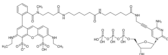
Structural formula of 5-Propargylamino-dCTP-ATTO-532-XX
