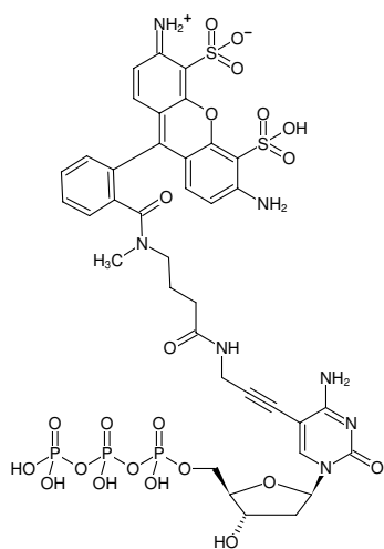
Structural formula of 5-Propargylamino-dCTP-ATTO-488
