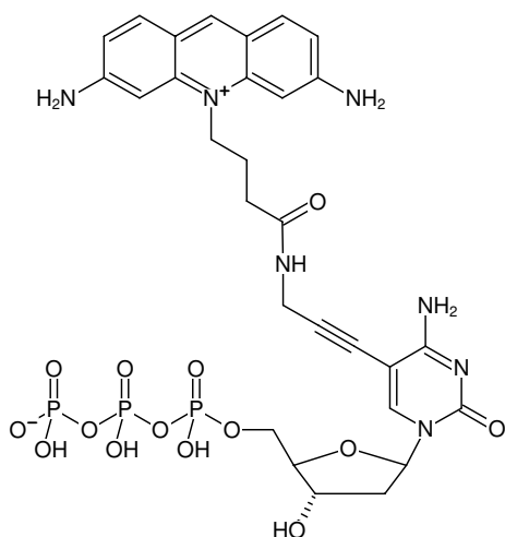
Structural formula of 5-Propargylamino-dCTP-ATTO-465
