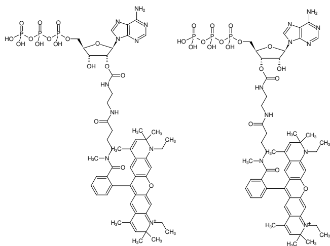
Structural formula of EDA-ATP-ATTO-Rho13
