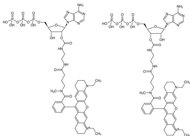
Structural formula of EDA-ATP-ATTO-Rho11
