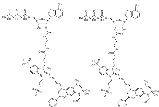
Structural formula of EDA-ATP-DY-776
