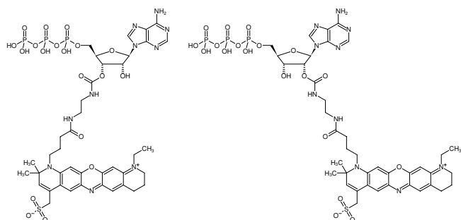
Structural formula of EDA-ATP-ATTO-680
