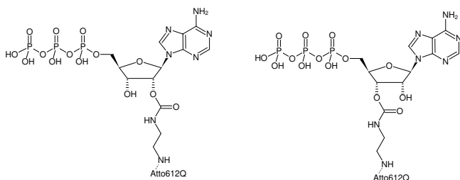
Structural formula of EDA-ATP-ATTO-612Q
