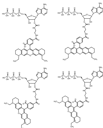
Structural formula of EDA-ATP-ATTO-565
