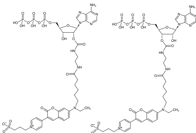
Structural formula of EDA-ATP-DY-485XL
