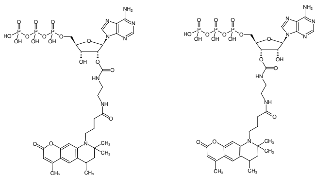
Structural formula of EDA-ATP-ATTO-390
