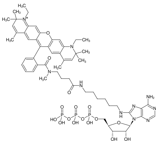
Structural formula of 8-(6-Aminoethyl)-amino-ATP-ATTO-Rho13
