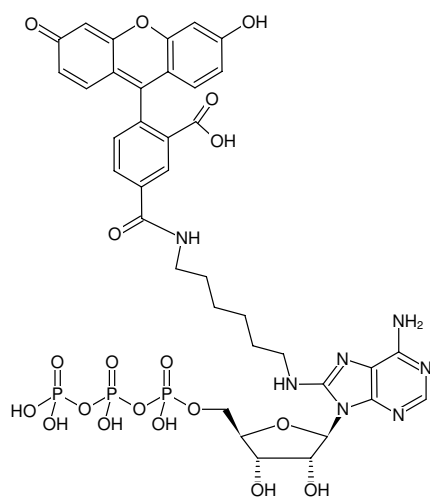
Structural formula of 8-(6-Aminoethyl)-amino-ATP-5-FAM
