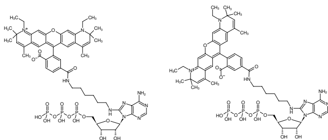
Structural formula of 8-(6-Aminoethyl)-amino-ATTO-590
