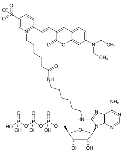
Structural formula of 8-(6-Aminoethyl)-amino-ATP-DY-480XL
