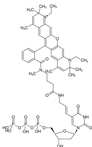
Structural formula of Aminoallyl-dUTP-ATTO-Rho13
