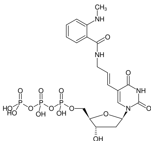
Structural formula of Aminoallyl-dUTP-MANT
