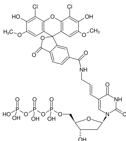
Structural formula of Aminoallyl-dUTP-6-JOE
