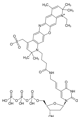
Structural formula of Aminoallyl-dUTP-ATTO-700
