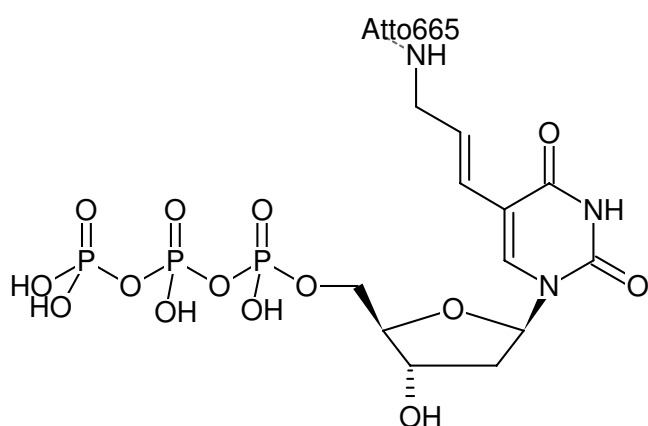
Structural formula of Aminoallyl-dUTP-ATTO-665
