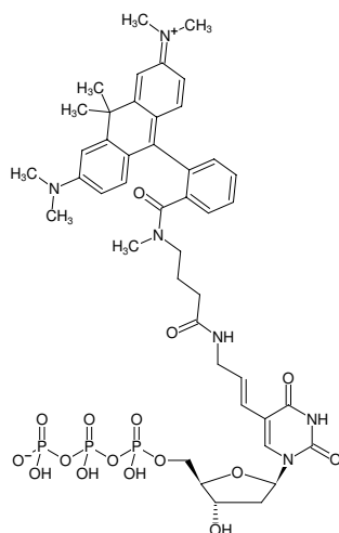
Structural formula of Aminoallyl-dUTP-ATTO-620
