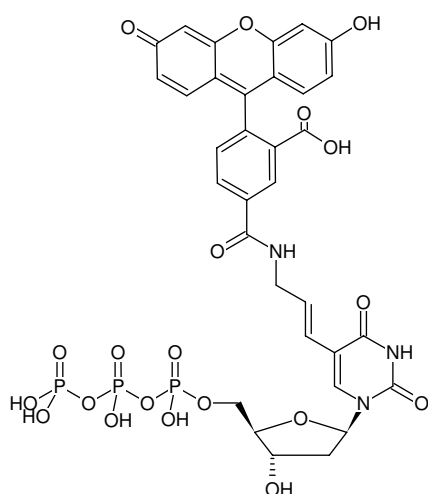
Structural formula of Aminoallyl-dUTP-5-FAM
