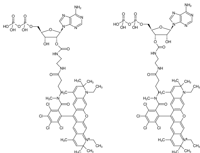
Structural formula of EDA-ADP-ATTO-Rho14
