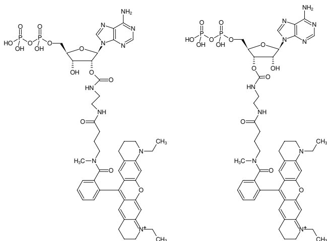
Structural formula of EDA-ADP-ATTO-Rho11
