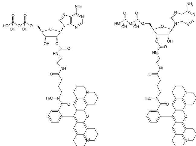
Structural formula of EDA-ADP-ATTO-Rho101
