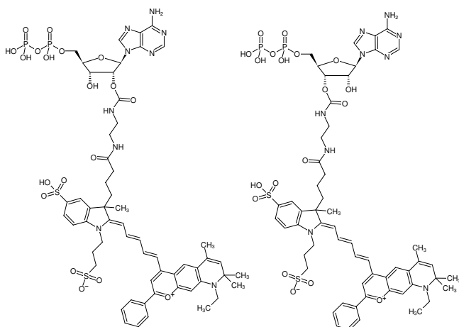
Structural formula of EDA-ADP-DY-776
