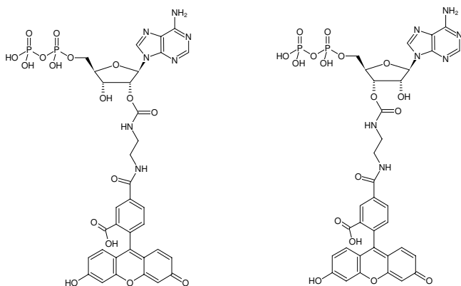
Structural formula of EDA-ADP-5-FAM
