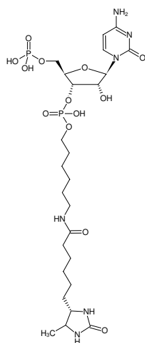
Structural formula of pCp-Desthiobiotin
