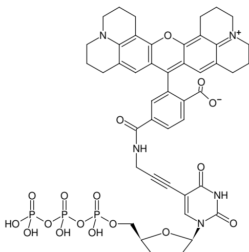
Structural formula of 5-Propargylamino-ddUTP-6-ROX
