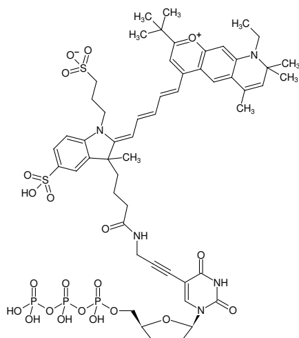
Structural formula of 5-Propargylamino-ddUTP-DY-751
